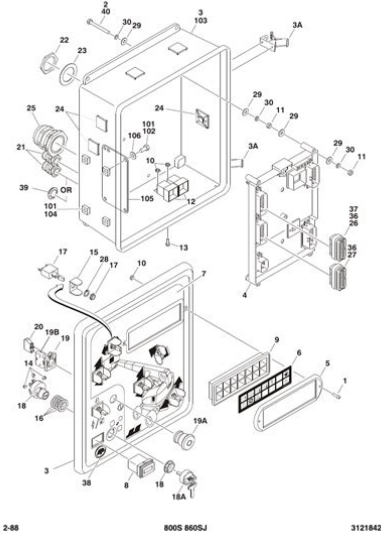
FIGURE 2-19. GROUND CONTROL BOX ASSEMBLY (WITHOUT UGM)
